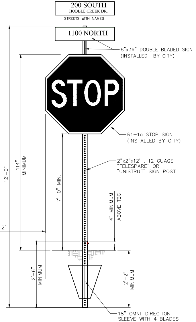
TYPICAL STREET/STOP SIGN INSTALLATION SCALE: 1"=2'
