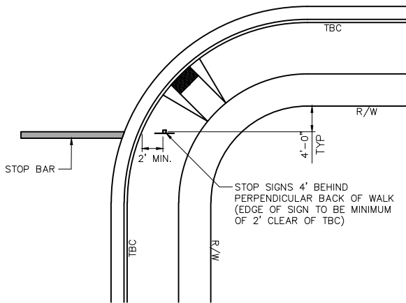
TYPICAL STREET/STOP SIGN LOCATION PLAN VIEW SCALE: 1"=20'
